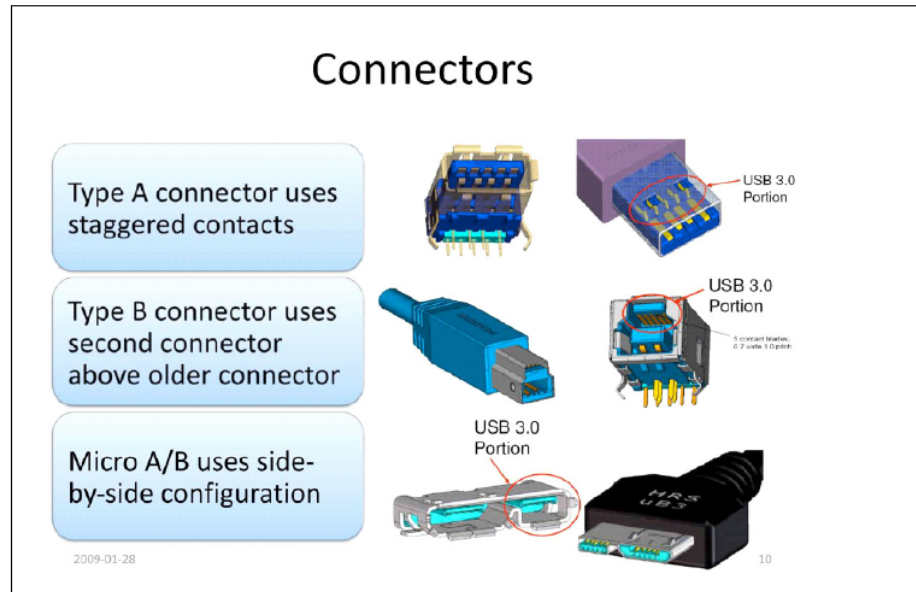
Figure 13: USB connector types
