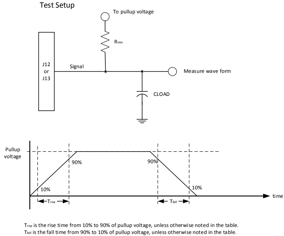
Figure 10: Test setup to determine the termination and conditioning values
