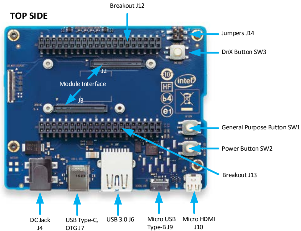
Figure 3. Intel Joule expansion board - top view
